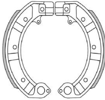
176.0128 ORIGINAL Ø 150 x 24 176.0128/R FOR RACE Ø 150 x 24
