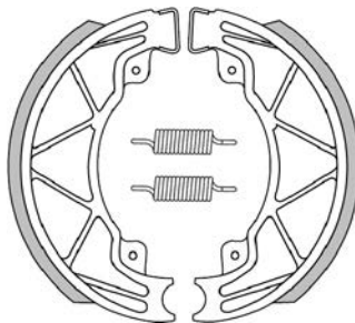
176.0300 ORIGINAL Ø 140 x 25 176.0300/R FOR RACE Ø 140 x 25
