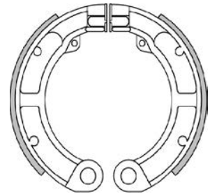
176.0130 ORIGINAL Ø 125 x 20
